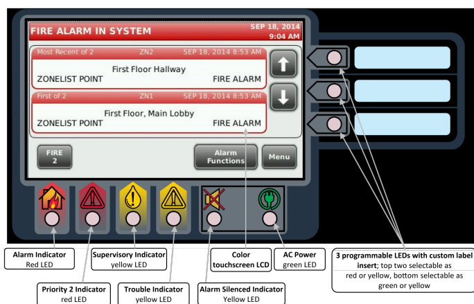
Figure 2: Touchscreen Display with LED Status Indicators
