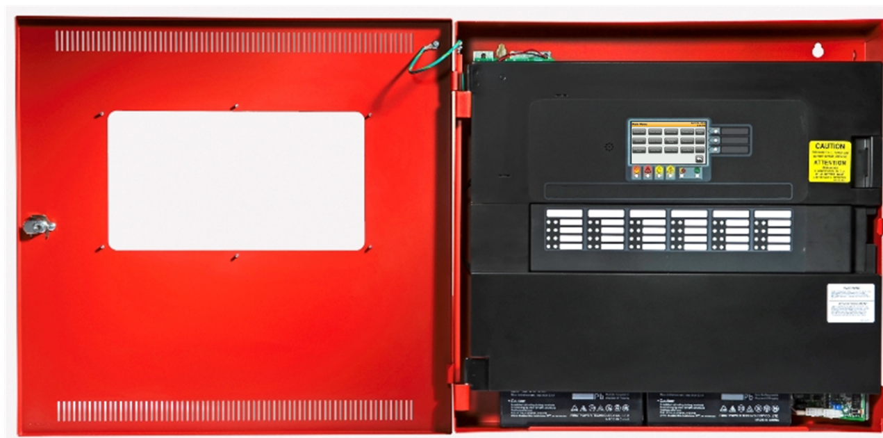
Figure 11: 4007ES with IDNAC Notification Operator View with door open
