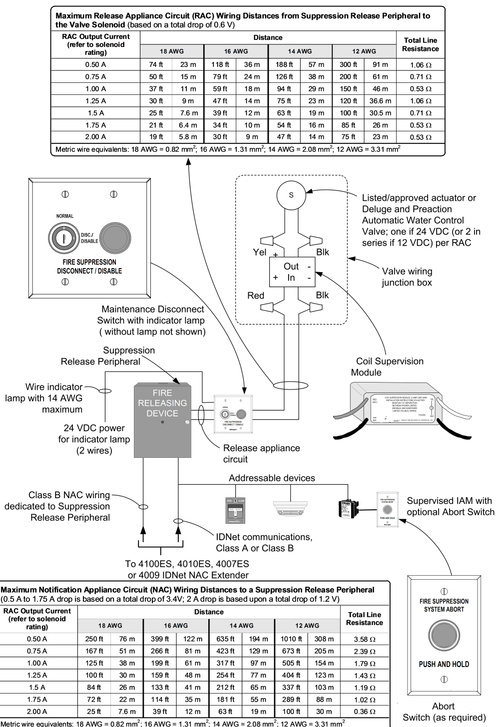
Fig 4: Suppression Release Peripheral Wiring Reference
