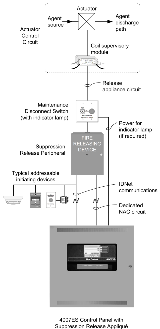
Fig 1: 4007ES Series Releasing Control Typical Block Diagram
