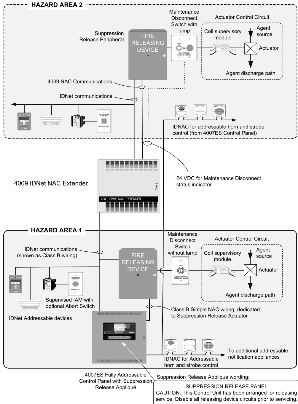
Fig 3: 4007ES Fully Addressable Panel Releasing System One-Line Connection Reference
