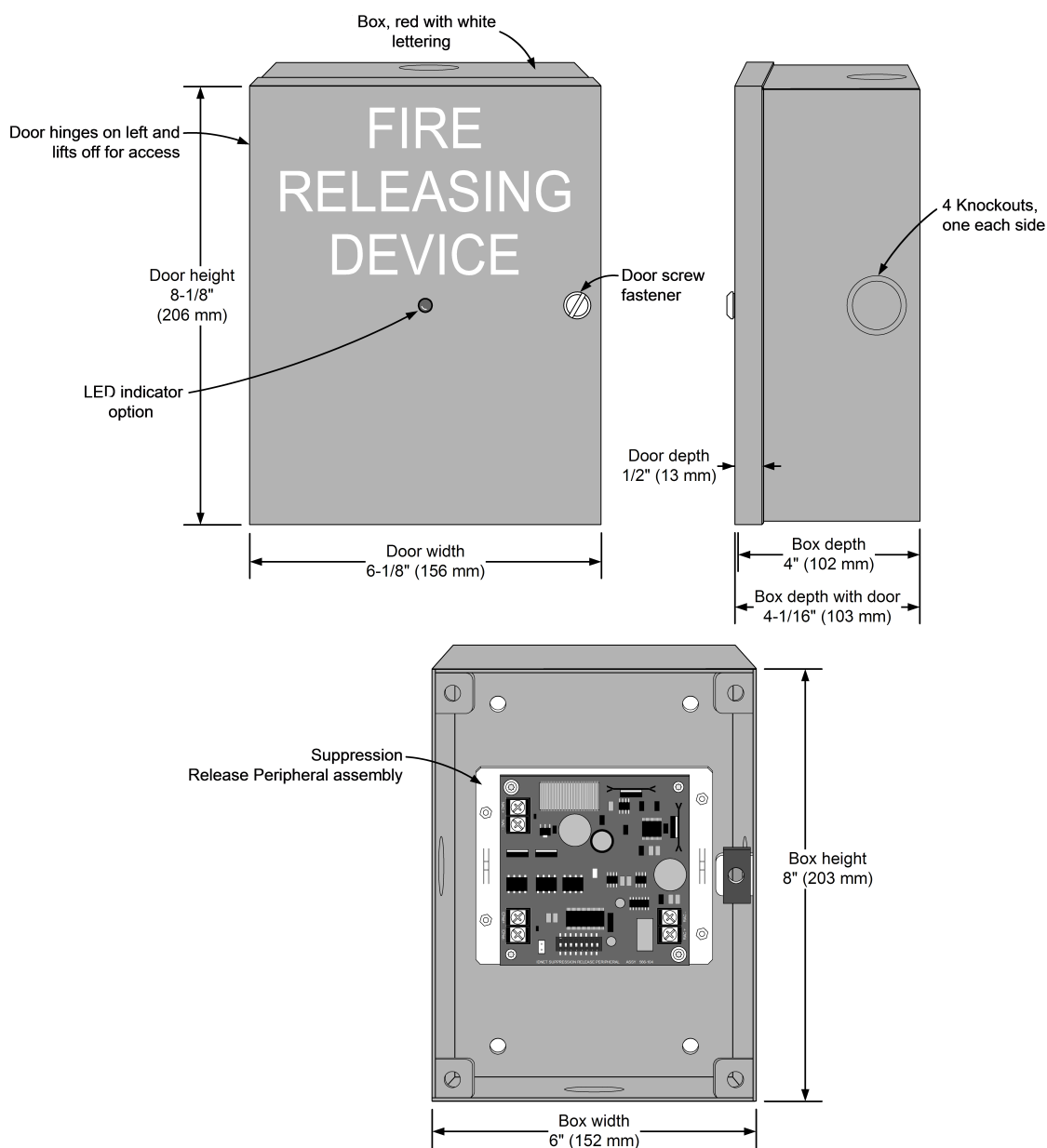
Fig 5: Suppression Release Peripheral Installation Reference Diagram
