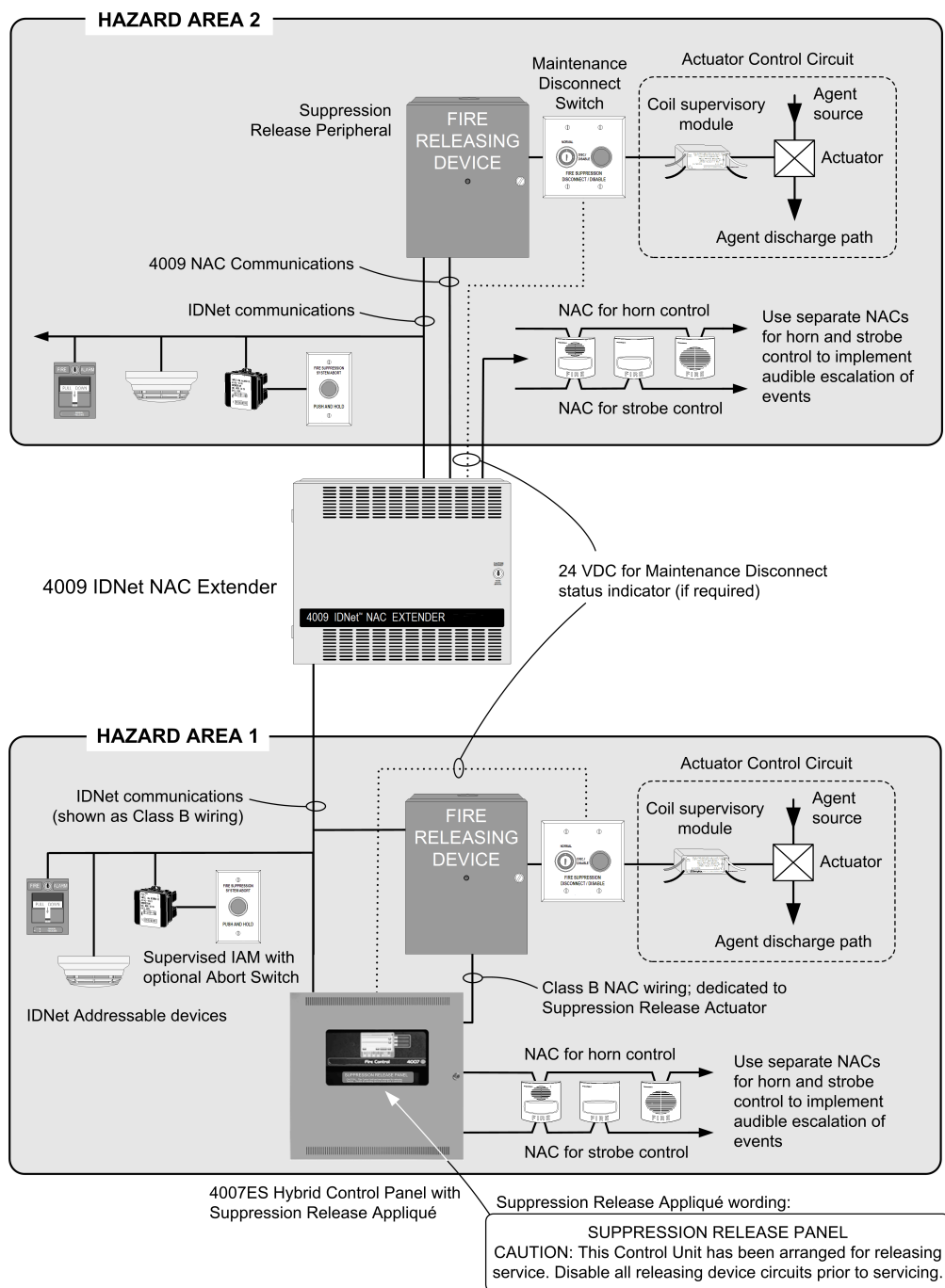
Fig 2: 4007ES Hybrid Panel Releasing System One-Line Connection Reference
