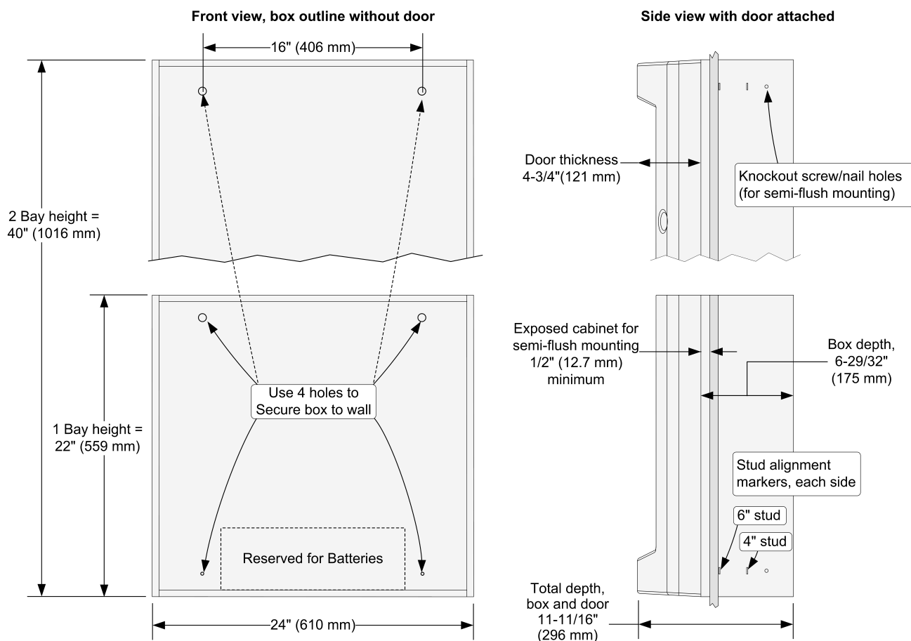
Figure 3: Cabinet Dimension Reference
