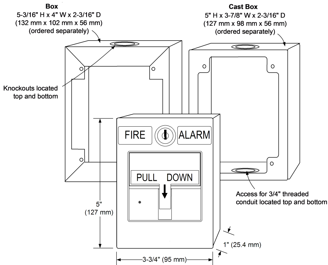
Fig 2: A4099 Series Addressable Manual Station
