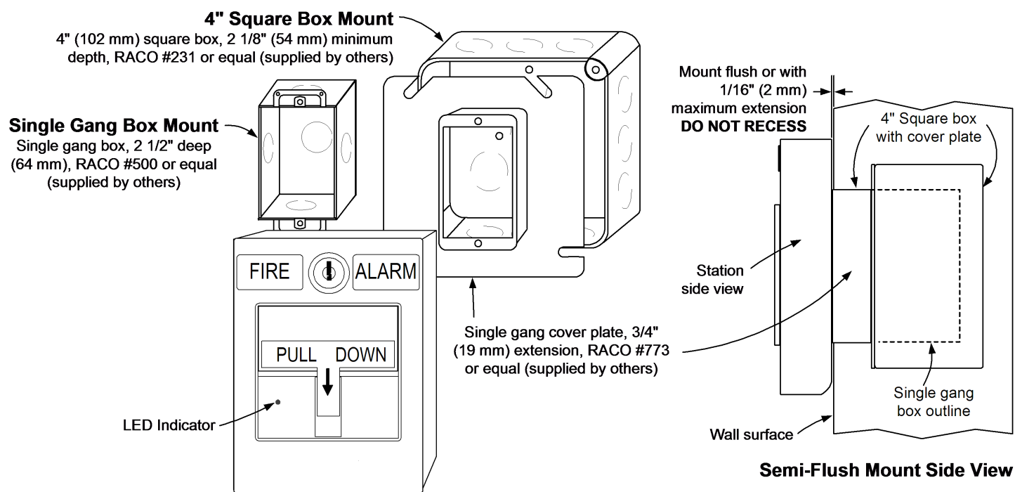
Fig 1: Addressable Manual Station Semi-Flush Mounting
