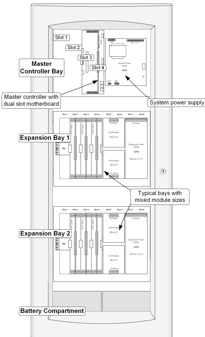
Figure 2: 4100ES Module Bay Reference
