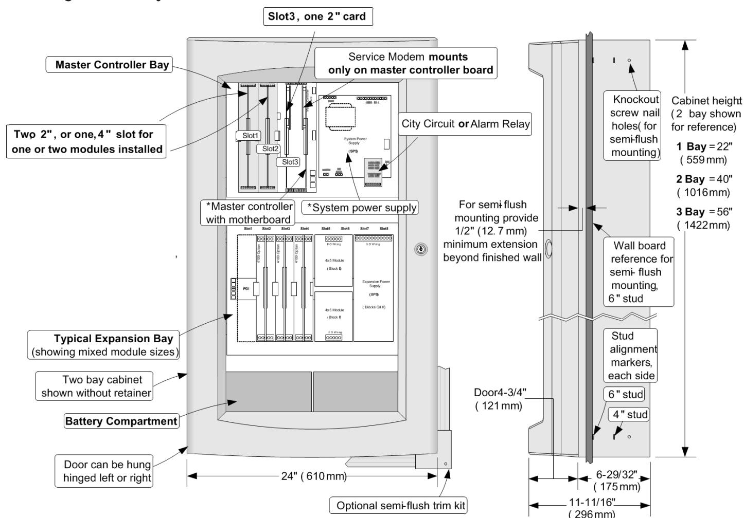
Figure 3: Mounting and CPU Bay Module Reference
