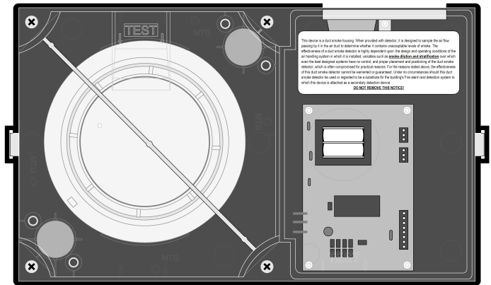
Fig 1: A4098-9687 Stand-Alone Duct Detector Housing, Front View
